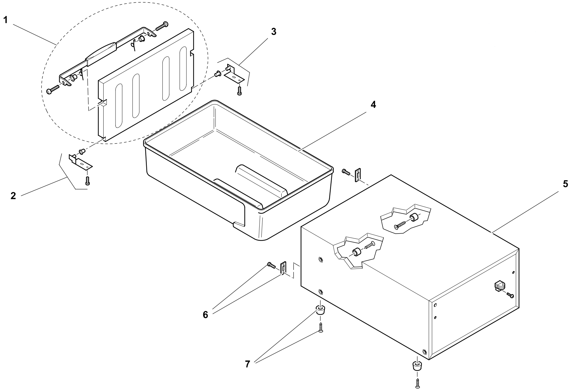
CR 36 - CABINET
